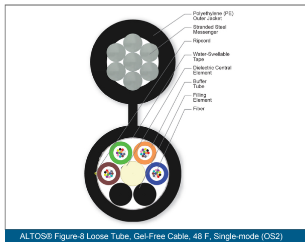
ALTOS® Figure-8 Loose Tube, Gel-Free Cable, 48 F, Single-mode (OS2)
