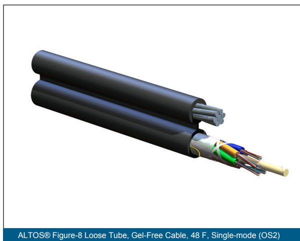
ALTOS® Figure-8 Loose Tube, Gel-Free Cable, 48 F, Single-mode (OS2)
